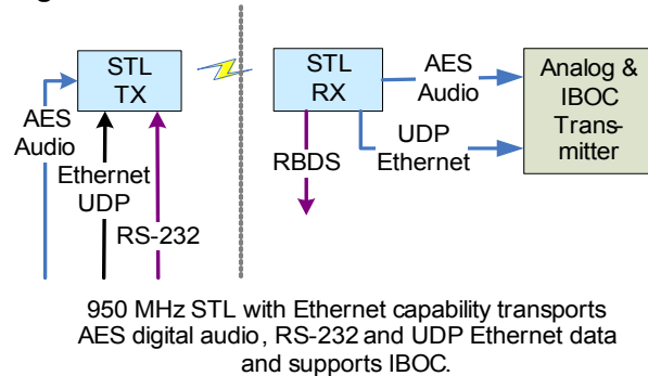
Figure 2: A 950 MHz STL with Ethernet
