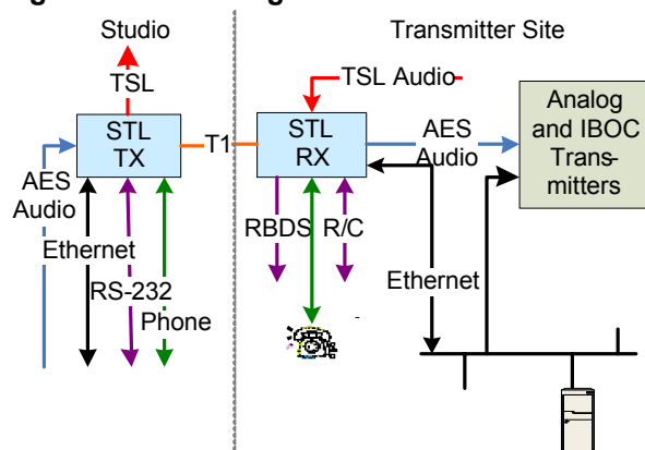
Figure 4: Block Diagram of a T1 STL/TSL
