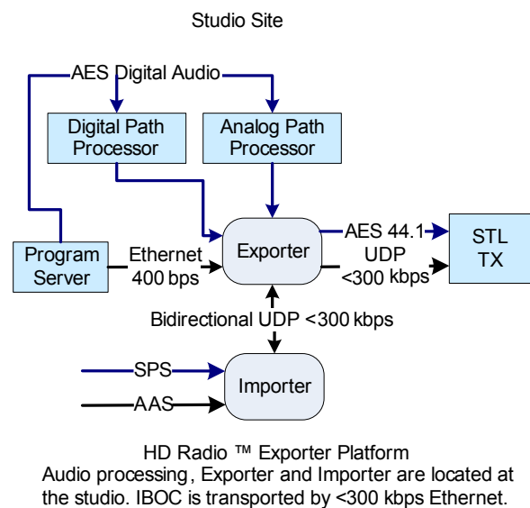
Figure 1: HD Radio™ Exporter Platform
