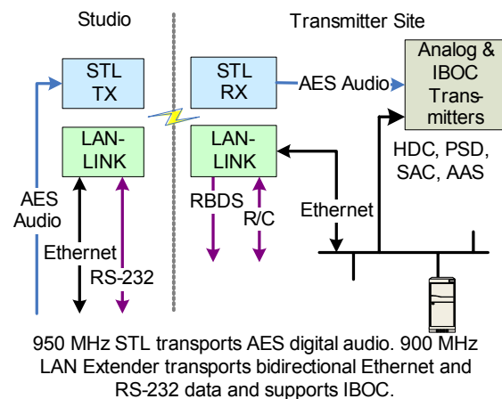
Figure 3: 950 MHz STL with 900 MHz LAN Extender/Data Link
